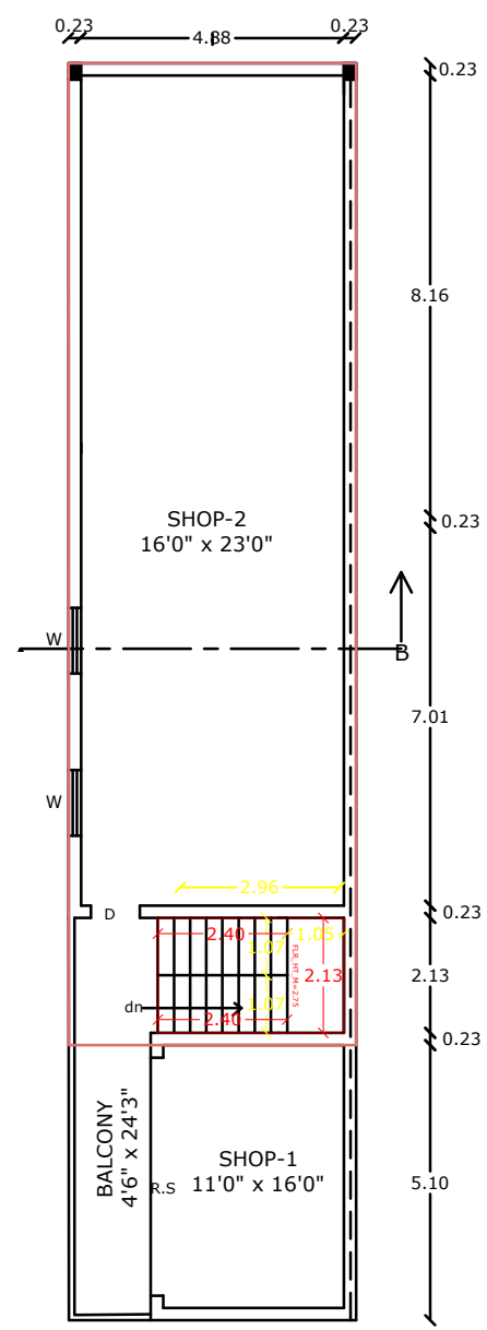
EXG.FIRST FLOOR PLAN
