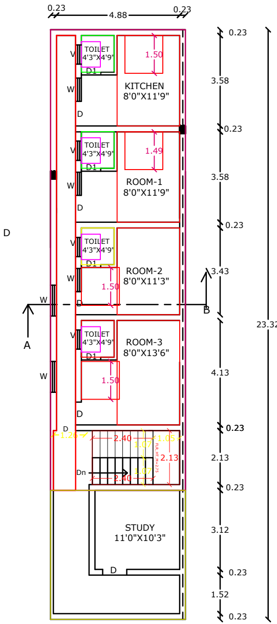
PRO.SECOND FLOOR PLAN
