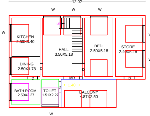
PROPOSED FF PLAN
