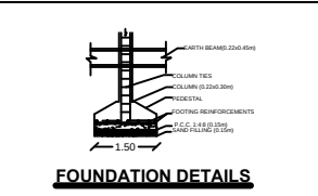
FOUNDATION DETAILS
