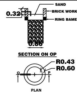
RAIN WATER PIT
