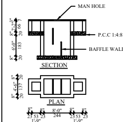
SEPTIC-TANK DETAIL
