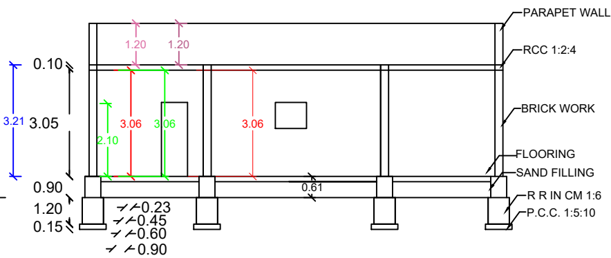
SECTION AB
