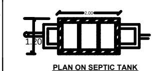
PLAN ON SEPTIC TANK
