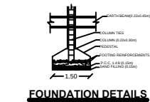
FOUNDATION DETAILS
