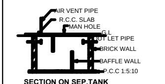
SECTION ON SEP.TANK
