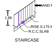
STAIRCASE
