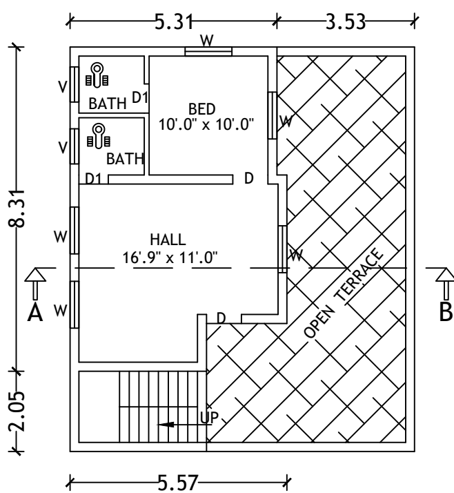
PLAN FIRST FLOOR
