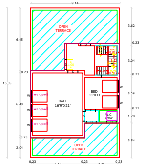
FIRST FLOOR RESIDENTIAL PLAN
