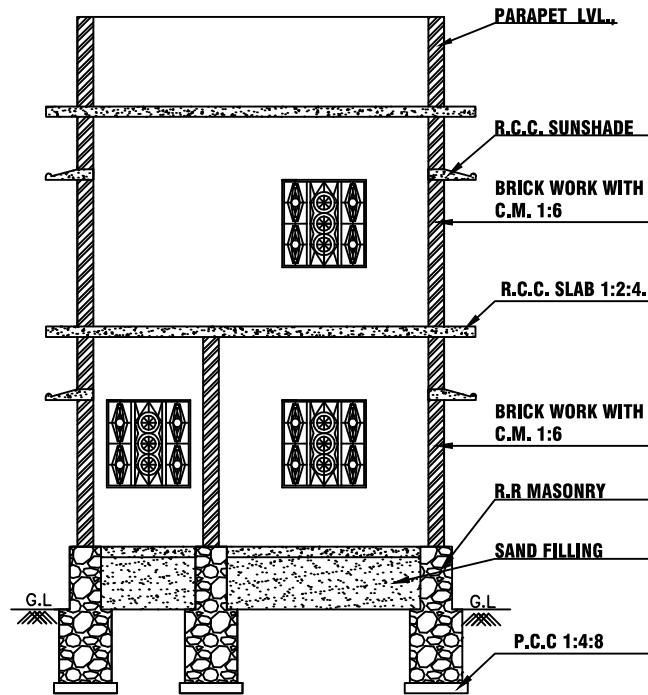
SECTION ON A-A & A'-A'
