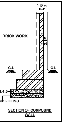
SECTION OF COMPOUND WALL
