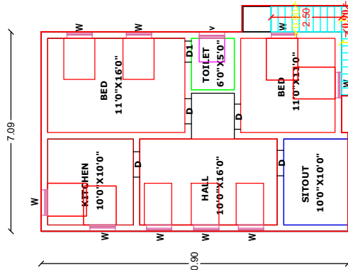
EXG.GROUND FLOOR PLAN
