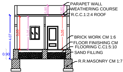
SECTION ON SV
