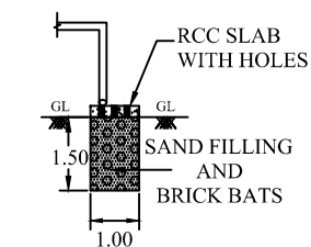
SECTION OF BS
