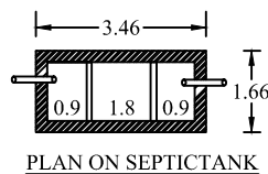
PLAN ON SEPTICTANK
