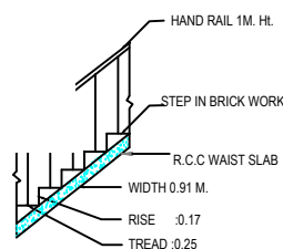
STAIR DETAIL
