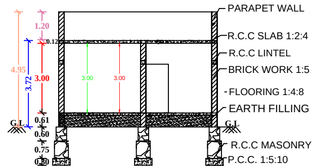
"SECTION "AB"
