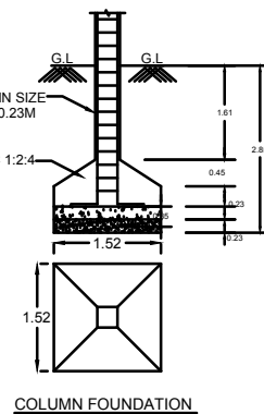
COLUMN FOUNDATION
