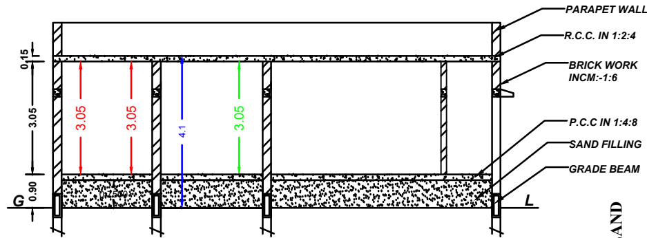
SECTION "AB"
