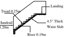
STAIRCASE DETAIL
