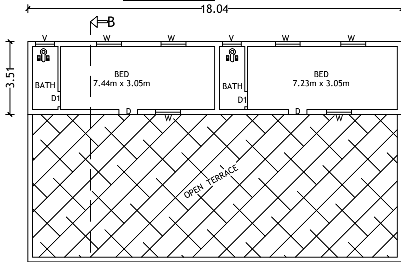
PLAN FIRST FLOOR
