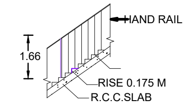
STAIRCASE
