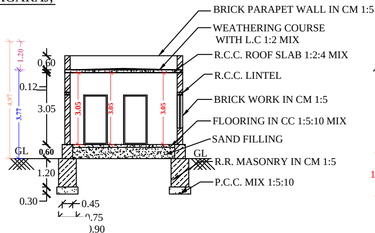
SECTION OF "AB"
