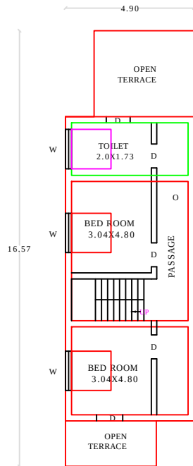
PROPOSED FF PLAN
