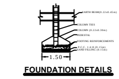
FOUNDATION DETAILS
