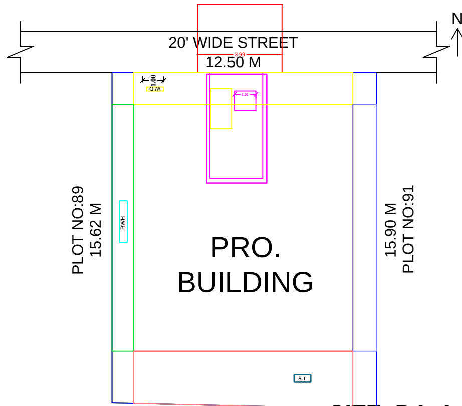
SITE PLAN
