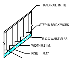
STAIR DETAIL
