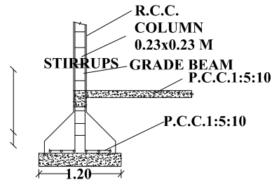
COLUMN DETAIL
