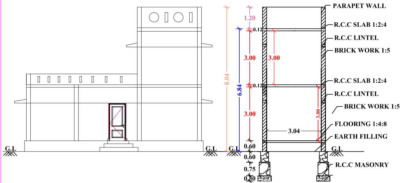
"FRONT ELEVATION"
