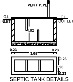
SEPTIC TANK DETAILS
