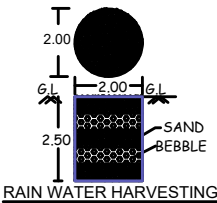
RAIN WATER HARVESTING
