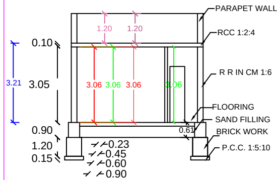
SECTION AB
