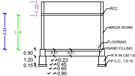
SECTION AB
