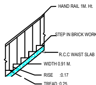
STAIR DETAIL
