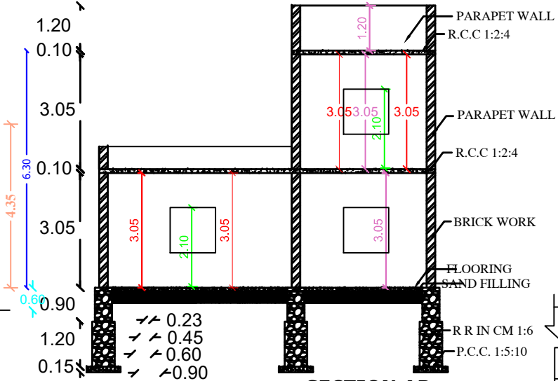
SECTION AB
