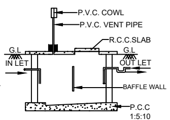
SEC. OF SEPTIC TANK
