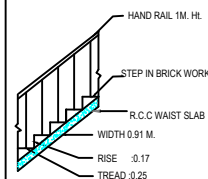
STAIR DETAIL
