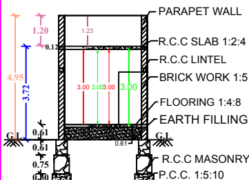
"SECTION "AB"
