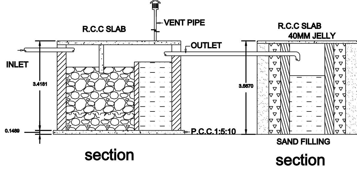
section
