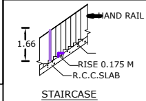
STAIRCASE
