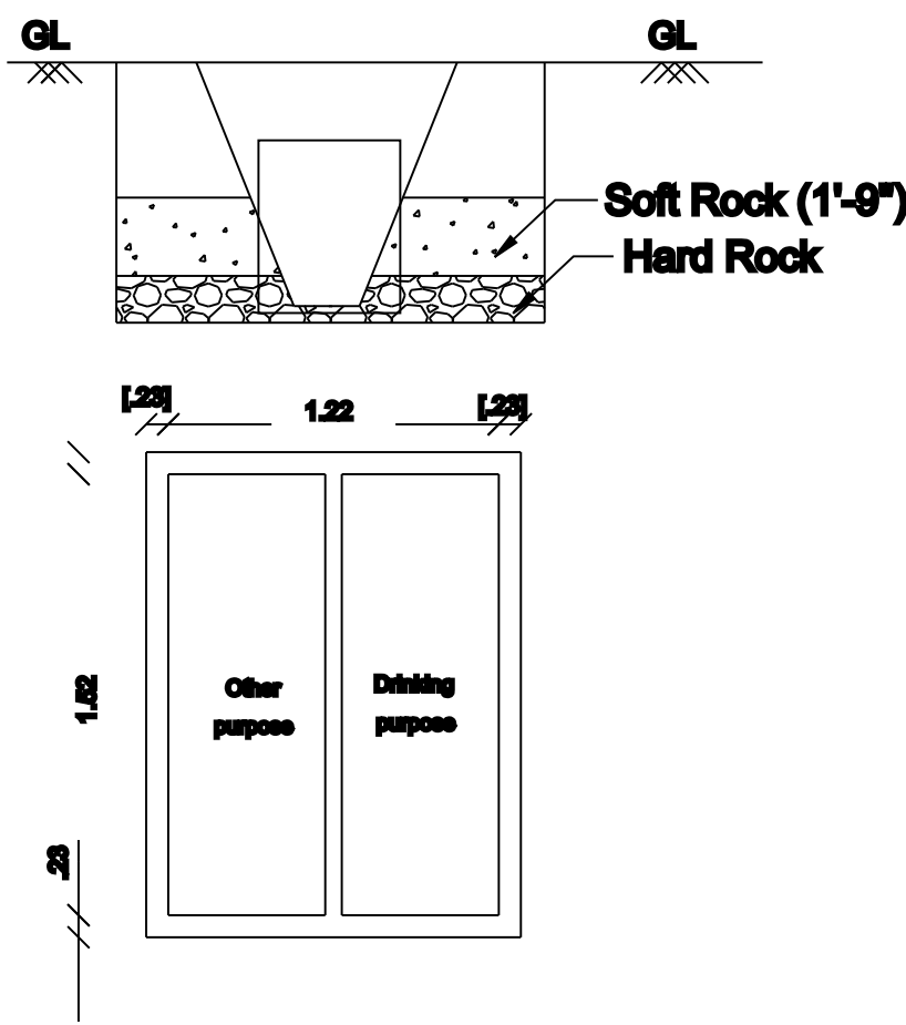
Over Head Tank Details
