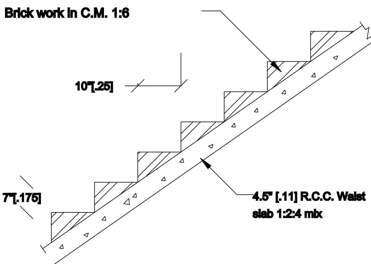
Staircase details ( Not to scale )
