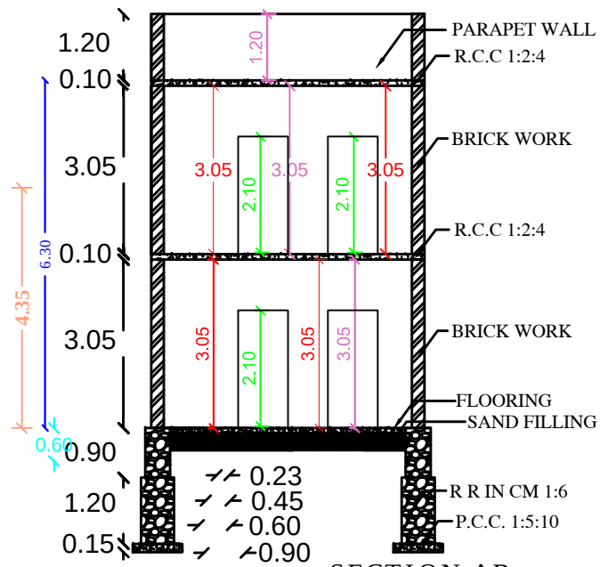
SECTION AB
