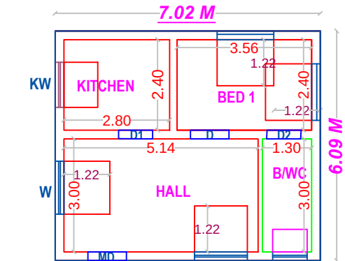
PLAN - GROUND FLOOR ( PROPOSED )
