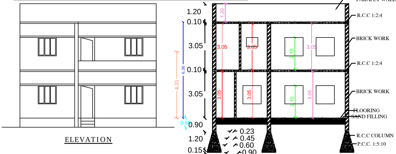
SECTION AB
