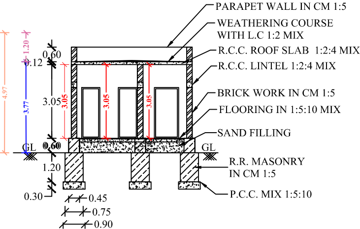
SECTION OF "AB"
