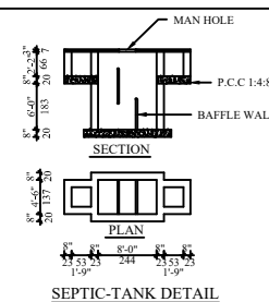
SEPTIC-TANK DETAIL
