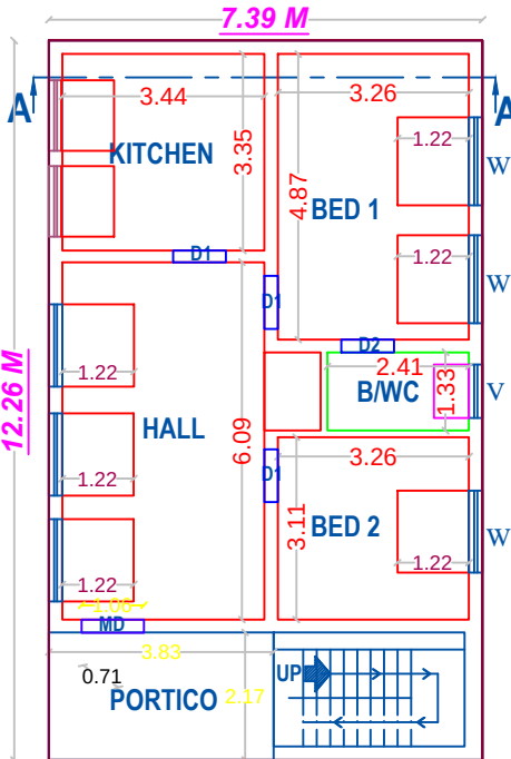
PLAN - GROUND FLOOR (PROPOSED)
