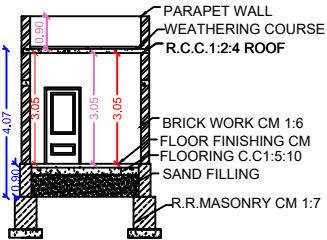
SECTION ON SV
