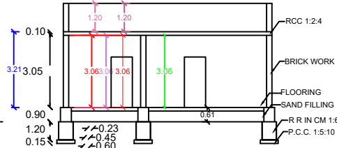
SECTION AB
