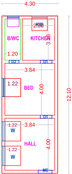
PLAN - GROUND FLOOR (PROPOSED)
