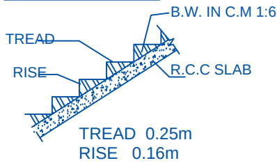
STAIR DETAILS
