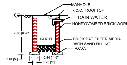
SECTION ON O - P
