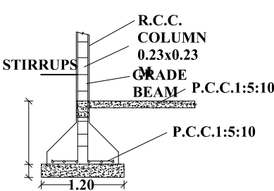
COLUMN DETAIL
