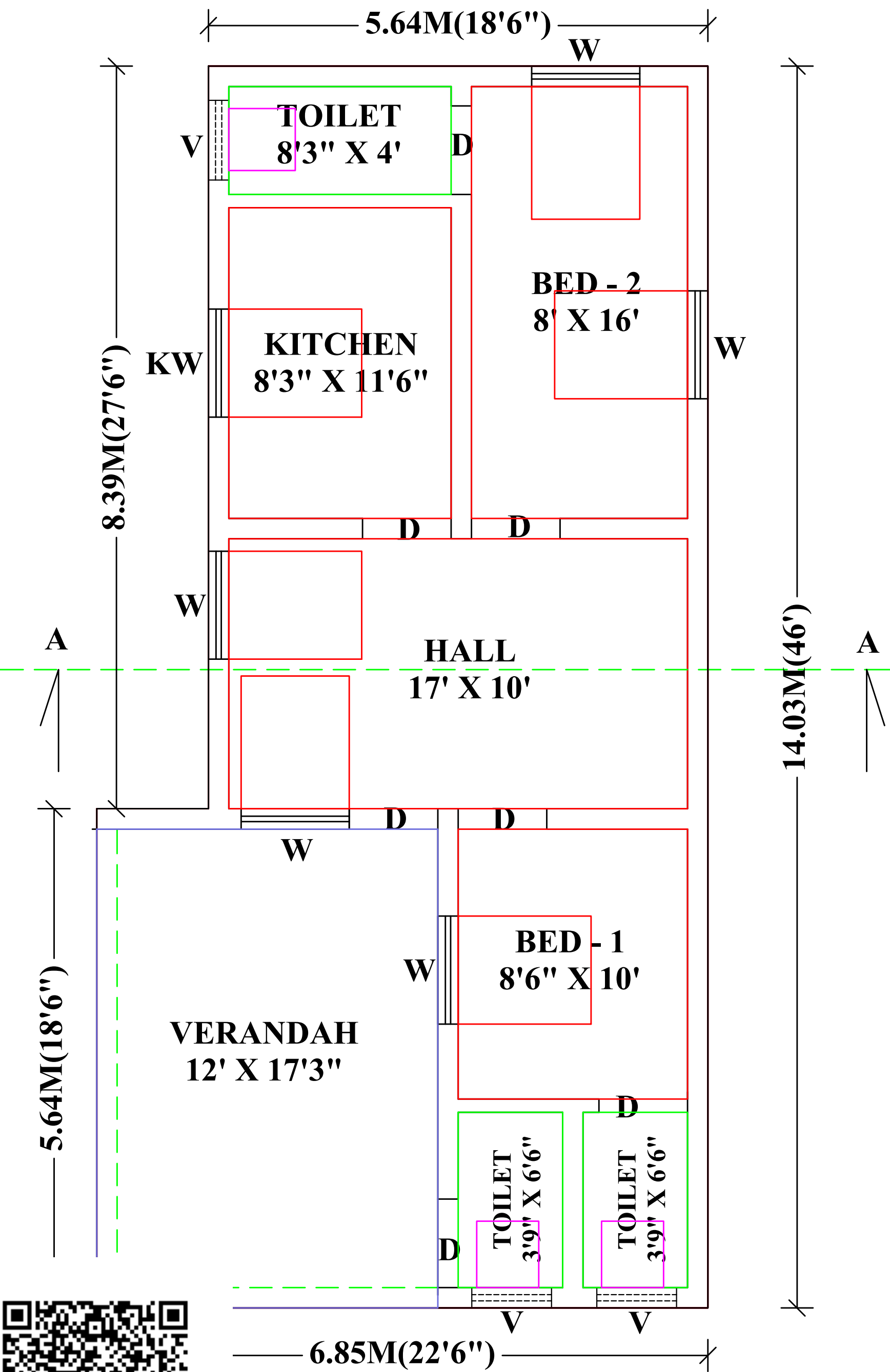
PLAN
