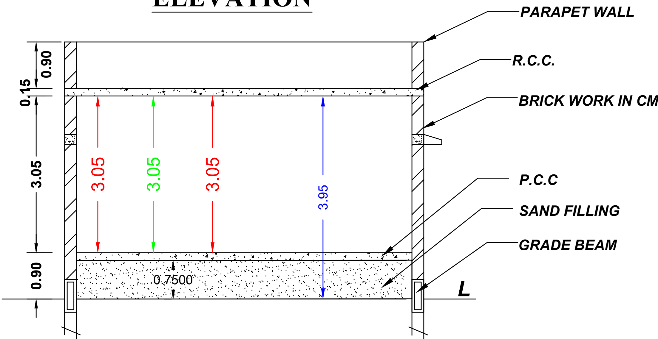
SECTION "AA"
