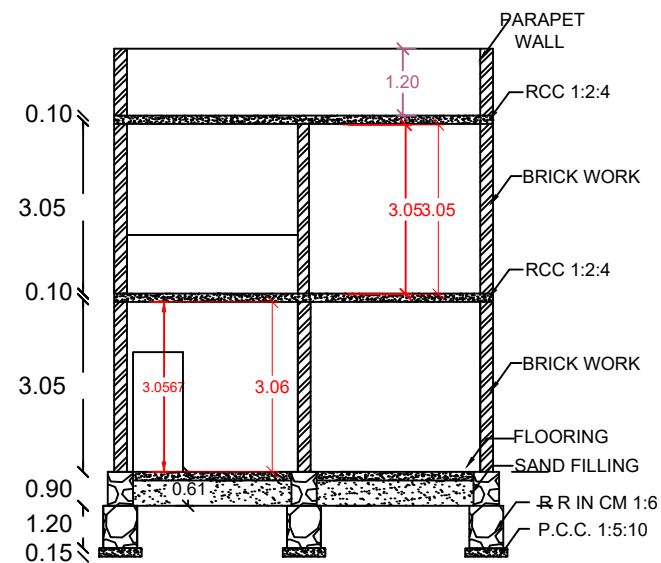
SECTION AB
