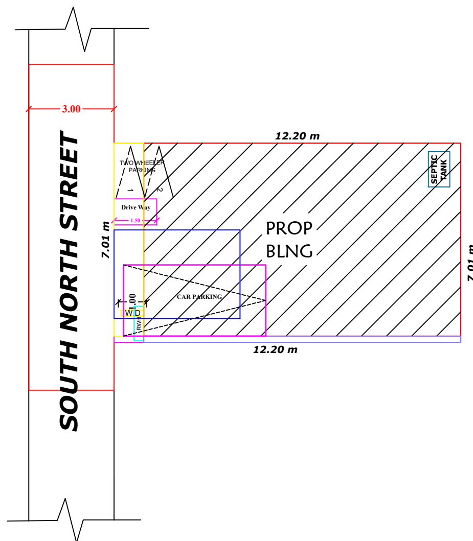
SITE PLAN
