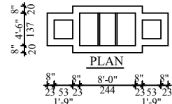
SEPTIC-TANK DETAIL
