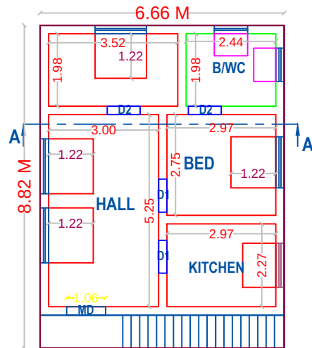
PLAN - GROUND FLOOR ( PROPOSED )
