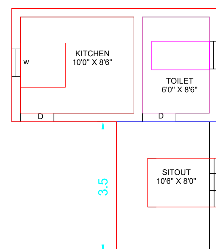
PROPOSED PLAN AC SHEET
