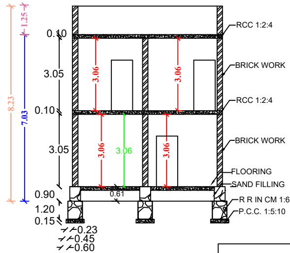
SECTION AB
