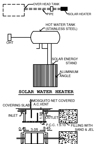
SEPTIC TANK & TRENCH U TRAP PROVISION
