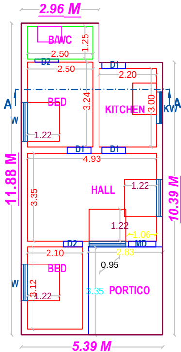
PLAN - GROUND FLOOR (PROPOSED)
